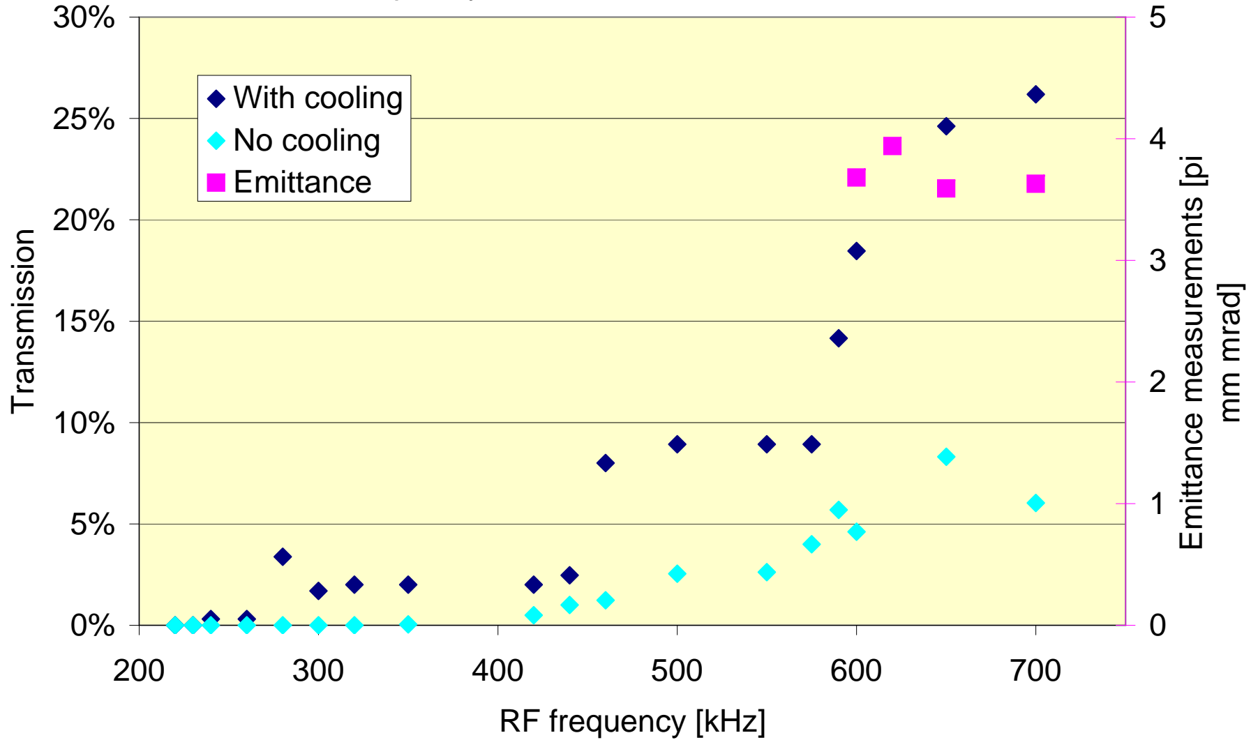
23-Na RF frequency influence on transmission and emittance
