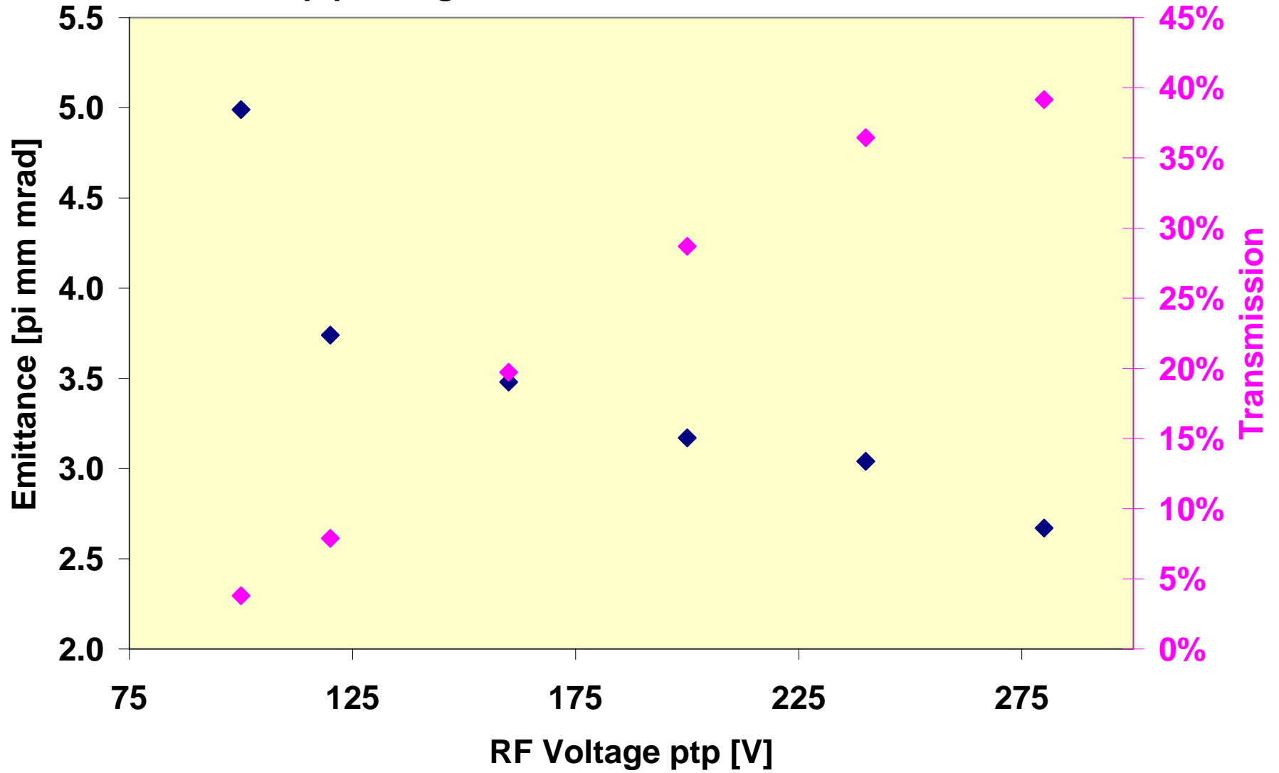
39-K RF ptp voltage influence on transmission and emittance
